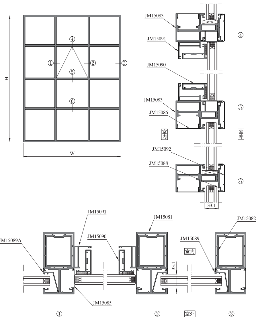
图中所示型材截面、装配、编号、尺寸及重量仅供参考。如有疑问，请向本公司查询。 Information above just for your reference. Please contact us if you have any questions, Thank you!
