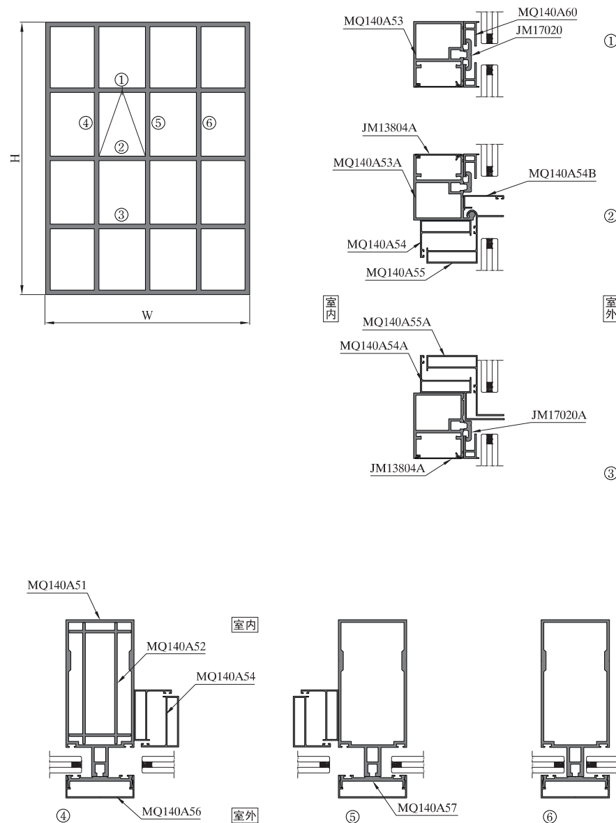
图中所示型材截面、装配、编号、尺寸及重量仅供参考。如有疑问，请向本公司查询。 Information above just for your reference. Please contact us if you have any questions, Thank you!
