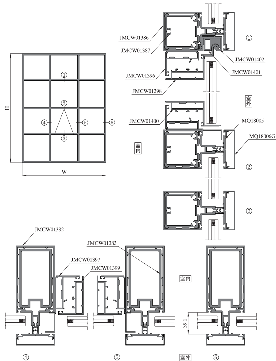
图中所示型材截面、装配、编号、尺寸及重量仅供参考。如有疑问，请向本公司查询。 Information above just for your reference. Please contact us if you have any questions, Thank you!
